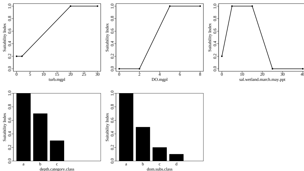
Figure 1. Suitability index graphs for variables included in the atlanticcroakerWetlandLATideLt0.5m model in ecorest .
